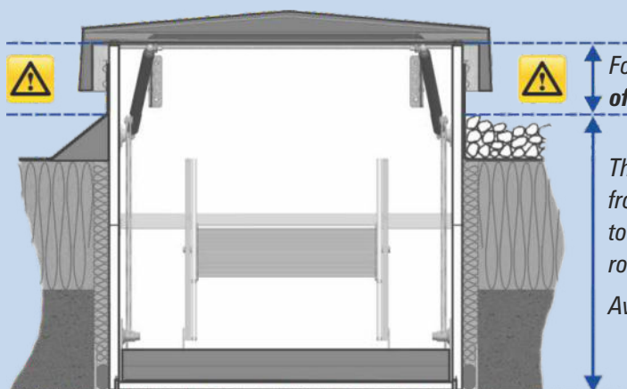
Fig.: Concertina attic stairs Liliput with thermal protection WS4D and flat roof exit
