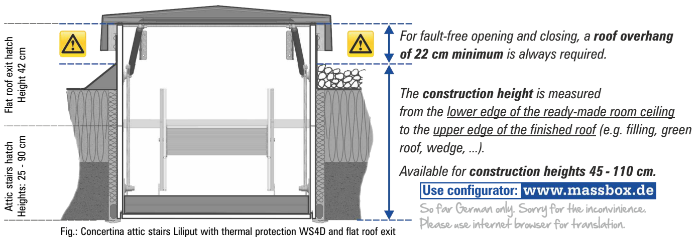
Fig.: Concertina attic stairs Liliput with thermal protection WS4D and flat roof exit
